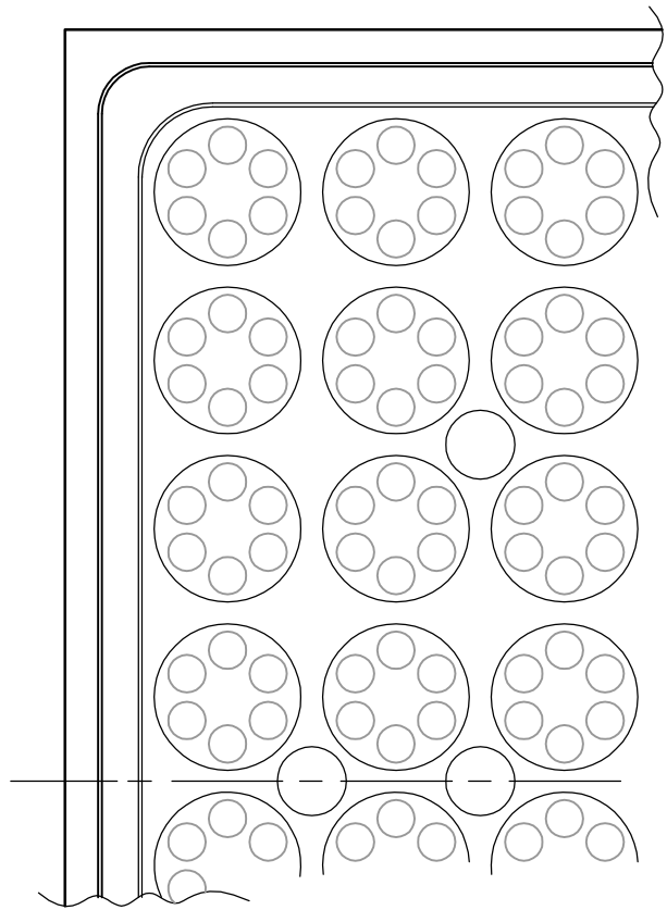
PARTIAL BOTTOM VIEW (Shown Without Optional Damper)
