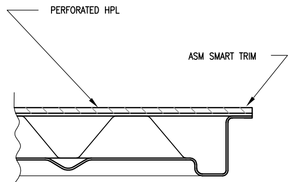
PARTIAL SECTION VIEW
